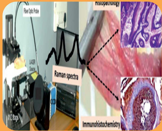
Raman spectroscopy in experimental oral carcinogenesis
